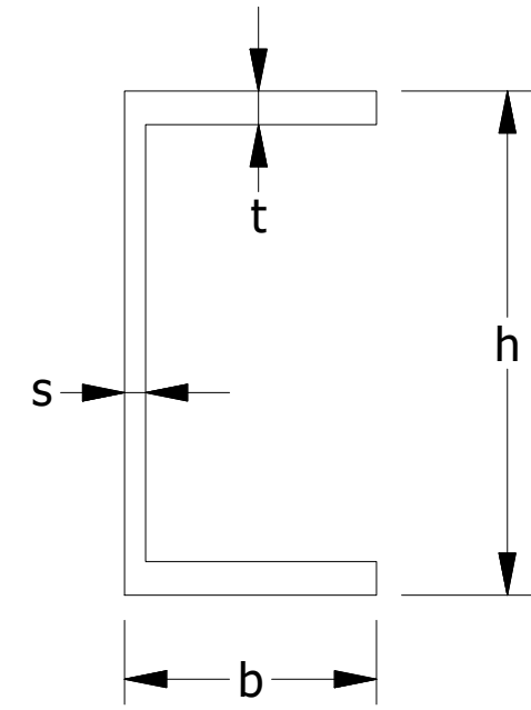
UPN
